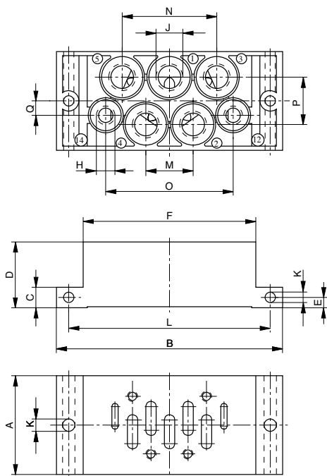
Dimensions (mm) Single Base Plate, Form B
